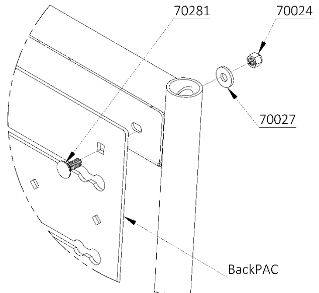
Figure 1: Installation Hardware
