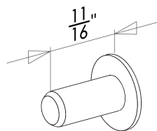
5/16-18 X 11/16" FLANGED BUTTON HEAD HEX DRIVE SCREW, SS, BLACK, w/ THREAD LOCKER [ITEM 18] {QTY. 48}
