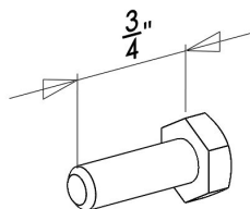
1/4-20 X 3/4" HEX HEAD SCREW, SS, BLACK [ITEM 23] {QTY. 16}
