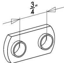
DOUBLE T-NUT, 15 SERIES, ECONOMY, 5/16-18 THREAD, SS [ITEM 11] {QTY. 8}
