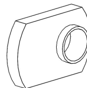
5/16-18 T-NUT, 15 SERIES, ECONOMY, SS, BLACK [ITEM 19] {QTY. 60}
