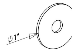
1/4" WASHER, 0.281" ID, 1" OD, SS, BLACK [ITEM 20] {QTY. 32}
