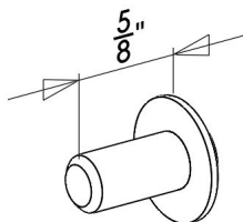
5/16-18 X 5/8" FLANGED BUTTON HEAD HEX DRIVE SCREW, SS, BLACK, w/ THREAD LOCKER [ITEM 24] {QTY. 26}
