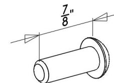
5/16-18 X 7/8" BUTTON HEAD HEX DRIVE SCREW, SS, BLACK, w/ THREAD LOCKER [ITEM 25] {QTY. 4}
