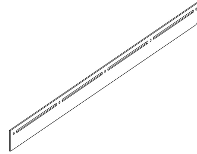
REAR SIDE PLATE [ITEM 4] {QTY. 2}
