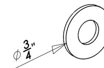
5/16" WASHER, 0.244" ID, 3/4" OD, SS, BLACK [ITEM 22] {QTY. 20}
