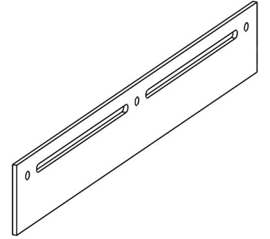
MIDDLE SIDE PLATE [ITEM 5] {QTY. 2}
