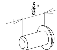
5/16-18 X 5/8" BUTTON HEAD HEX DRIVE SCREW, SS, BLACK, w/ THREAD LOCKER [ITEM 24] {QTY. 4}
