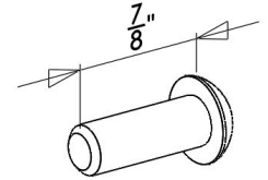
5/16-18 X 7/8" NON-FLANGED SCREW [ITEM 17] {QTY. 4}
