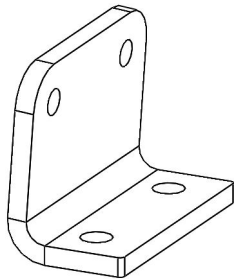
ROOF RACK BRACKET 8020 ADAPTER [ITEM 10] {QTY. 10}
