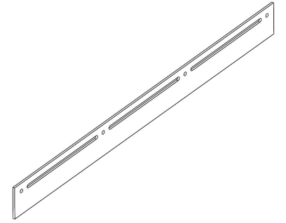
EXTENDED MIDDLE SIDE PLATE [ITEM 27] {QTY. 2}
