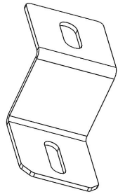
SOLAR PANEL BRACKET, FLUSH [ITEM 9] {QTY. 16}
