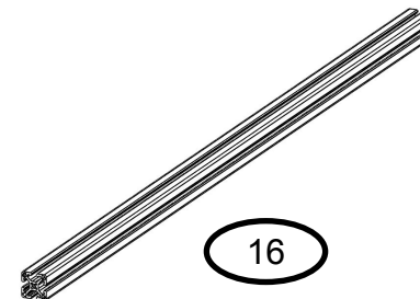
8020 SIDE RAIL-60.69" LG [ITEM 16] {QTY. 6} *One label per extrusion. 6 total
