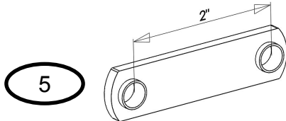
DOUBLE T-NUT, 2" SPACING [ITEM 5] {QTY. 12}
